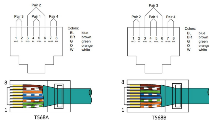
Figure 6: Eight-position jack pin-pair assignment T568A and T568B
