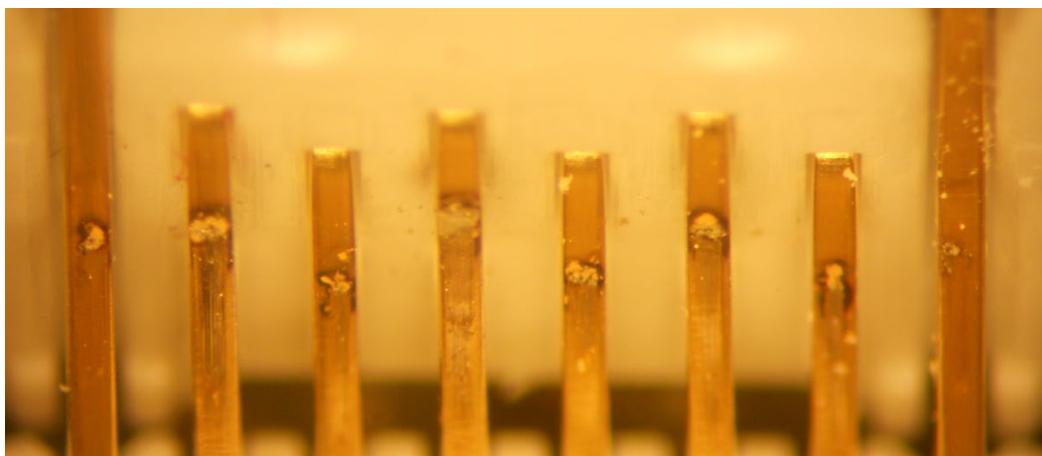
Figure 3: Unmating under PoE load causes an arc at the discharge area that can damage the plug and jack contacts.
