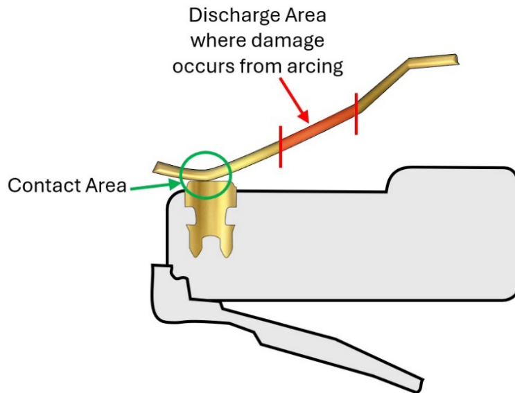
Figure 4: RJ45 connectors must ensure that damage from arcing remains in the discharge area and does not occur in the nominal contact area.
