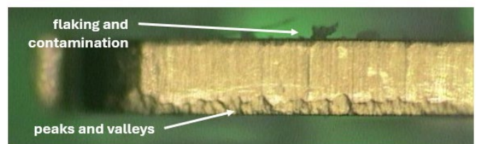
Poor Quality Wire Brushed RJ45 Contact
