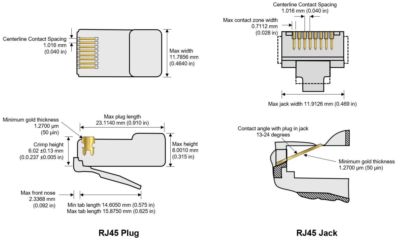
Figure 1: TIA-1096-A defines physical dimensions, mechanical characteristics, and contact material requirements for RJ45 plugs and jacks.
